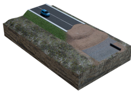
Rigid inclusions
