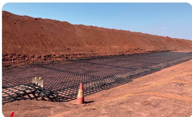
Mine soil reinforcement, Australia
